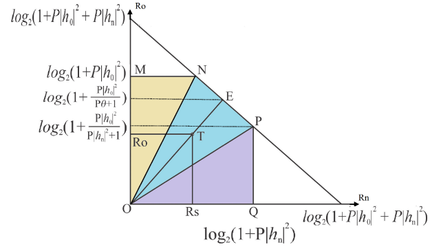
Fig. 2. The capacity region of RSMA.
